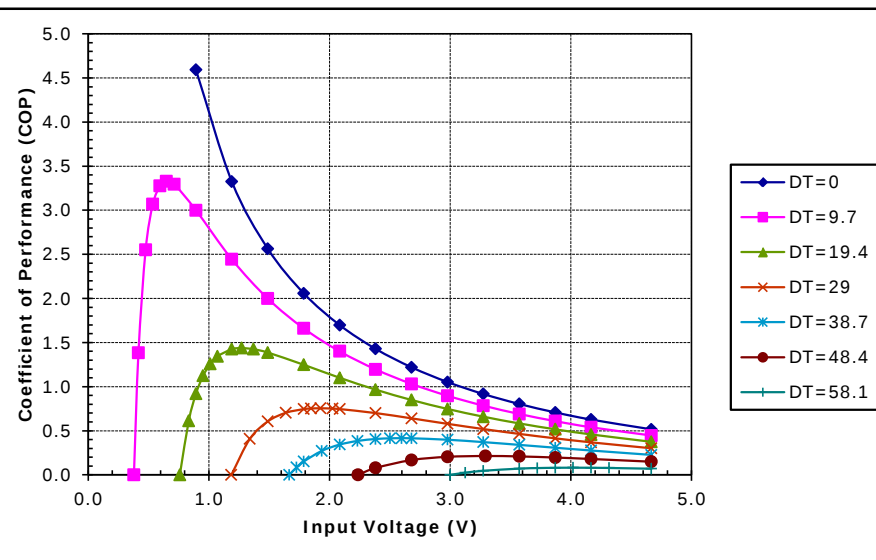
Unpotted CH-38-1.0-0.8 at a hot-side temperature of 30 °C
