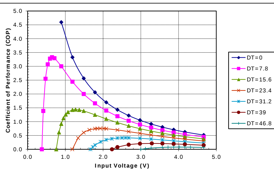
Potted CH-38-1.0-0.8 at a hot-side temperature of 30 °C
