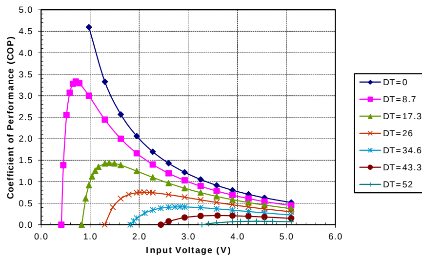
Potted CH-38-1.0-0.8 at a hot-side temperature of 50 °C
