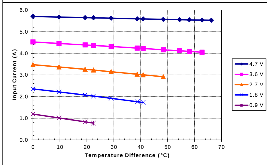
Unpotted CH-38-1.0-0.8 at a hot-side temperature of 30 °C
