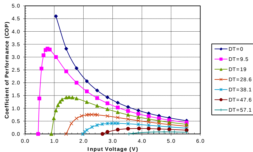
Potted CH-38-1.0-0.8 at a hot-side temperature of 70 °C
