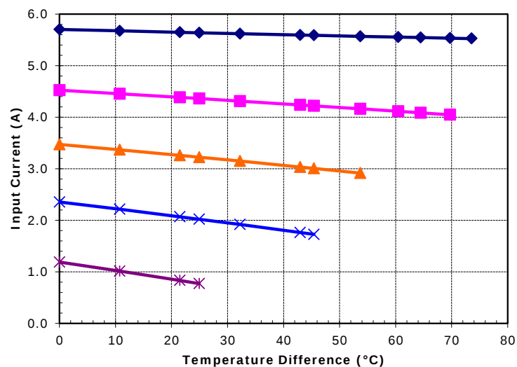
Unpotted CH-38-1.0-0.8 at a hot-side temperature of 50 °C
