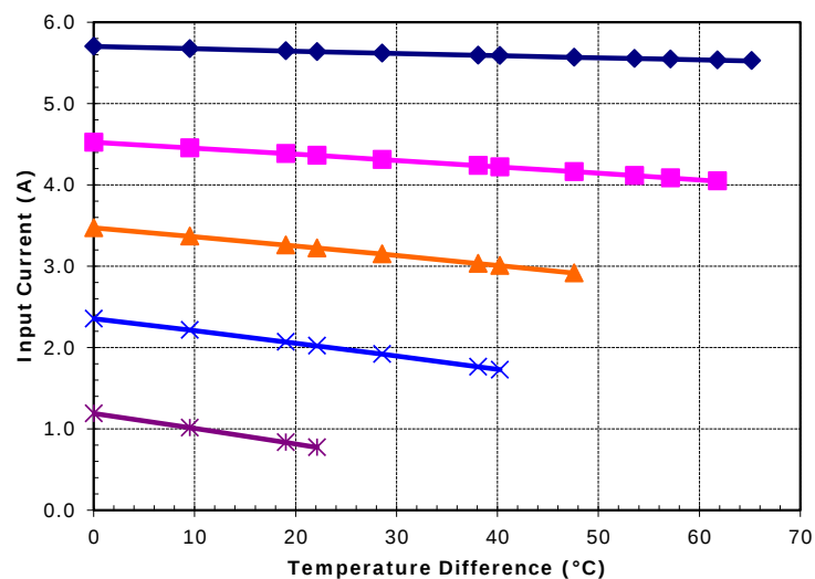
Potted CH-38-1.0-0.8 at a hot-side temperature of 70 °C
