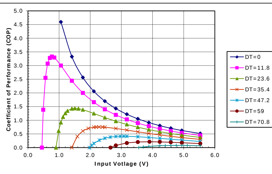
Unpotted CH-38-1.0-0.8 at a hot-side temperature of 70 °C
