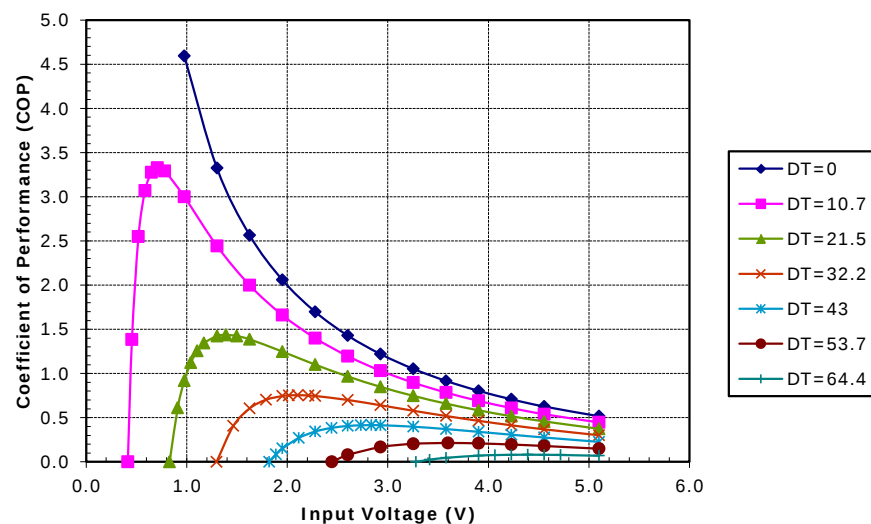
Unpotted CH-38-1.0-0.8 at a hot-side temperature of 50 °C
