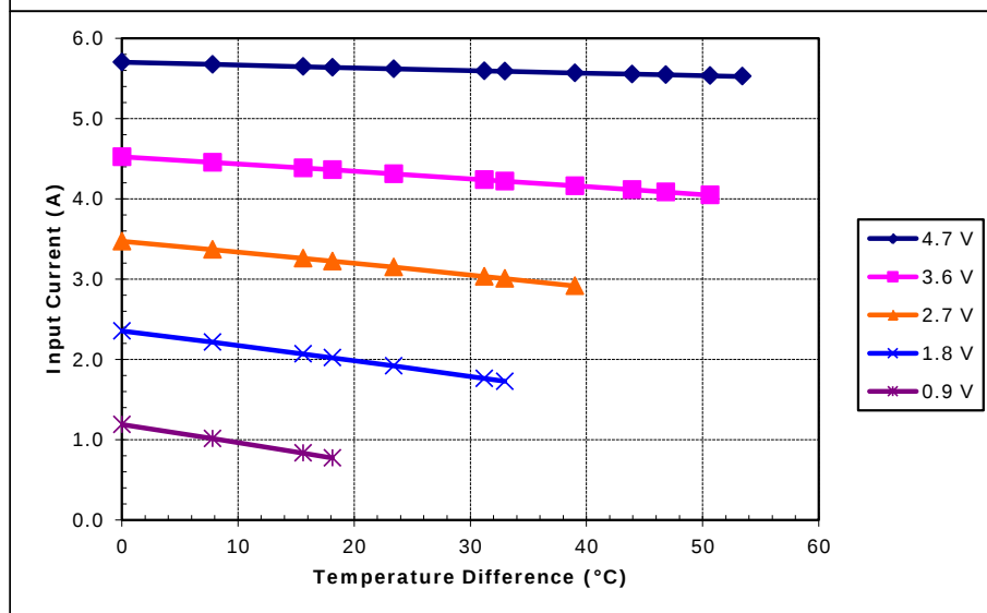
Potted CH-38-1.0-0.8 at a hot-side temperature of 30 °C
