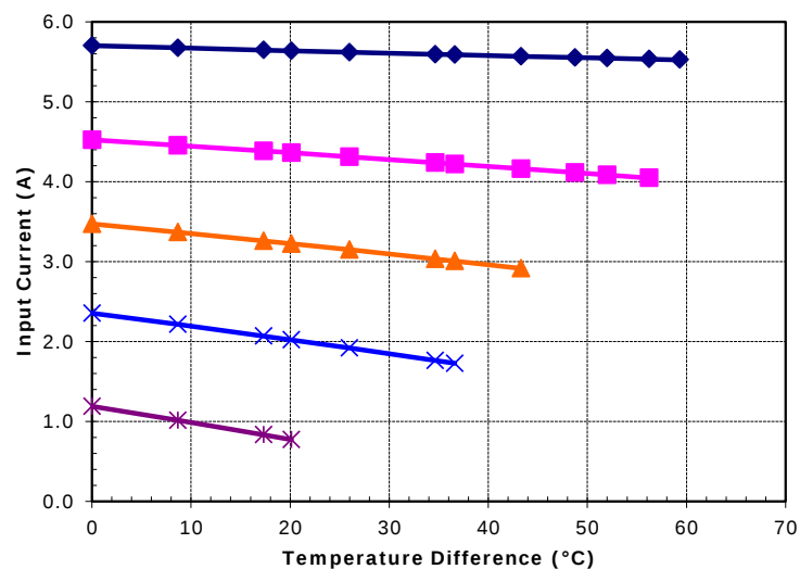
Potted CH-38-1.0-0.8 at a hot-side temperature of 50 °C
